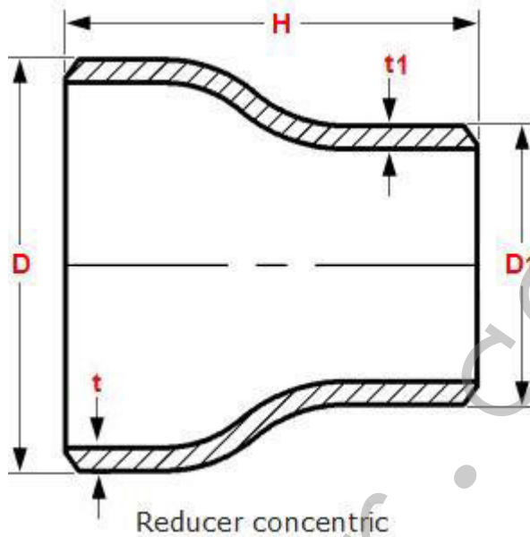
EEMUA 234 Concentric Reducer - Material Cu-Ni 90/10 and Cu-Ni 70/30
